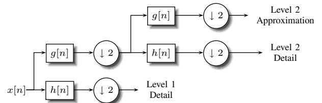
Fig. 2. Recursive Pyramidal Algorithm for Multi-Level Wavelet Transform
